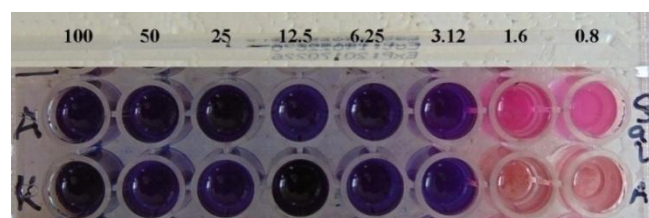
Figure 1: Microplate shows minimum inhibitory concentration of ethanol and dichloro methane extracts of Couroupita guianensis
